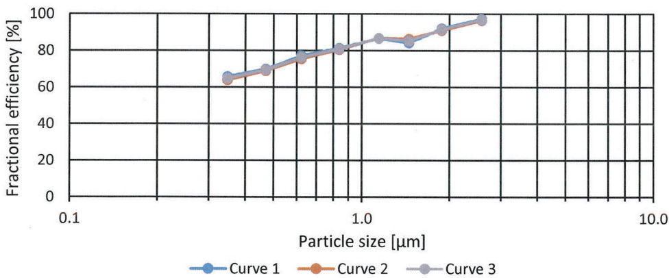
Test performed at 3400 m 3 /h - Speed air passage 4m/s
